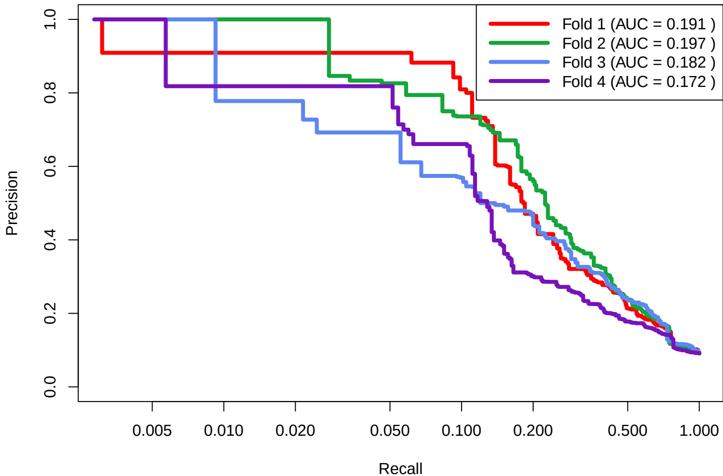
SPELL All Datasets: 430x20x1 Validation
